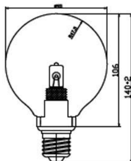
E27 Globe-cover Ø95 +48W ES G9 Item no. RX27G952B 95,0 x 95,0 x 14,0 cm Max. 70W - E27 - 240V Incl. G9 48W ES
