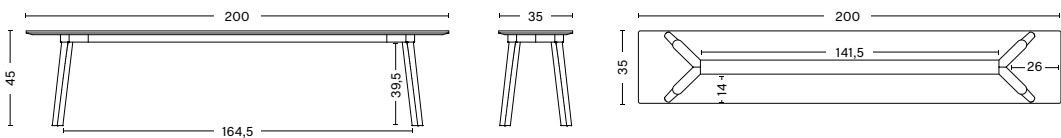
CPH DEUX 215 BENCH Length 200 cm Width 35 cm Height 45 cm
