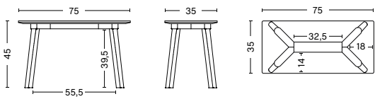
CPH DEUX 215 BENCH Length 75 cm Width 35 cm Height 45 cm
