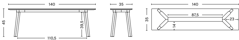
CPH DEUX 215 BENCH Length 140 cm Width 35 cm Height 45 cm
