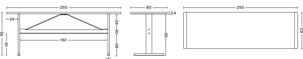
HIGH TABLE Width 250 cm Depth 80 cm Height 95 cm Crossbar height 48 cm
