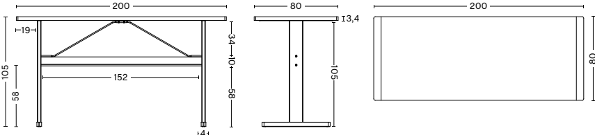
HIGH TABLE Width 200 cm Depth 80 cm Height 105 cm Crossbar height 58 cm
