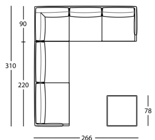
Nr. 9 = 1330/211S+1330/301TD+1330/PUF
