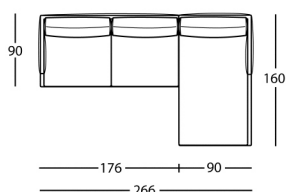
Nr. 5 = 1330/201S+1330/AL1D
