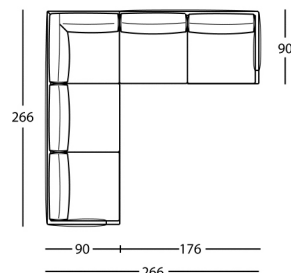
Nr. 2 = 1330/301TS+1330/201D
